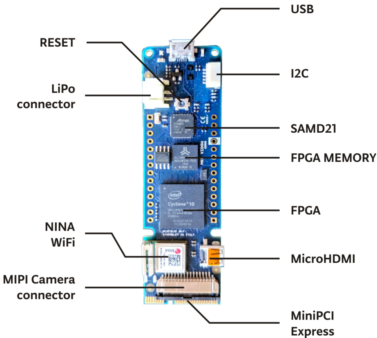
Board Overview
